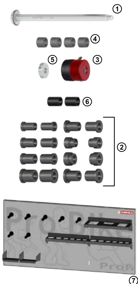
Upgrade kit for floating axles Item No. 815 008 002
