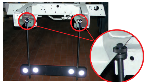
Clamping device of frame scale
