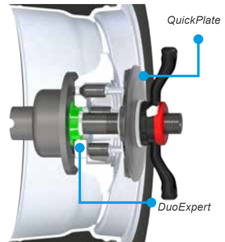
Mounting a wheel with the QuickPlate . The correct centring and clamping devices guarantee a perfect balancing result.
